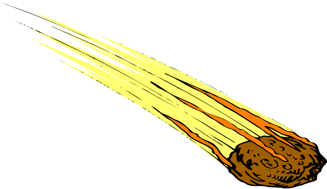
meteor
