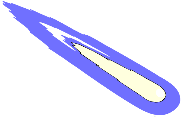
comet
