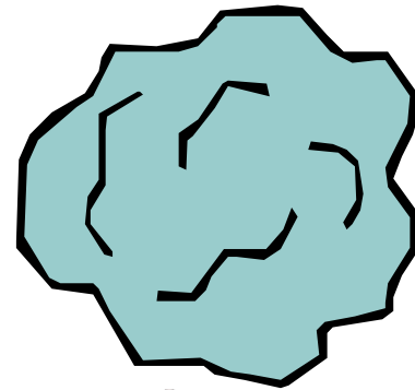
asteroid
