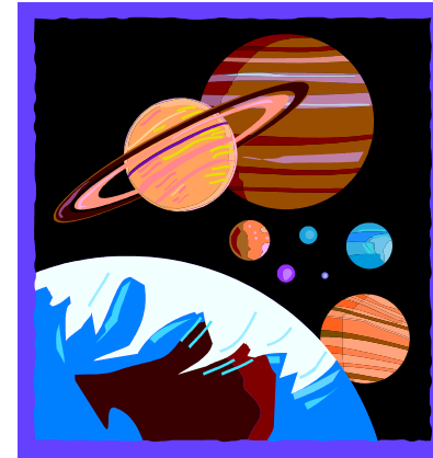
Solar System
